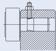
Fig. 8 Mounting example of Easy Mounting Type Cam Follower
